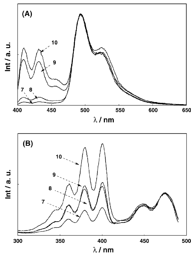
Fig. 4 (A) Fluorescence spectra ( \lambda_{\text{ex}} = 378 nm, normalized at 500 nm) and (B) excitation spectra of 7–10 ( \lambda_{\text{em}} = 500 nm, normalized at 470 nm) in chloroform solutions.
