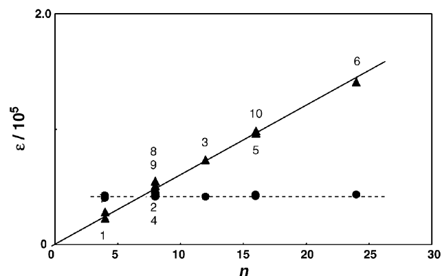
Fig. 3 Plots of extinction coefficients ( \epsilon ) at 359 nm (▲, solid line) and at 477 nm (●, dotted line) vs. the total number of anthracene units ( n ) for 1–10.
