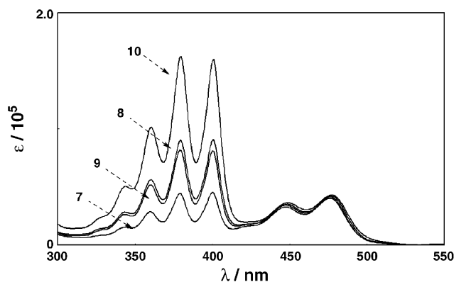
Fig. 2 Absorption spectra of 7–10 in chloroform solutions.
