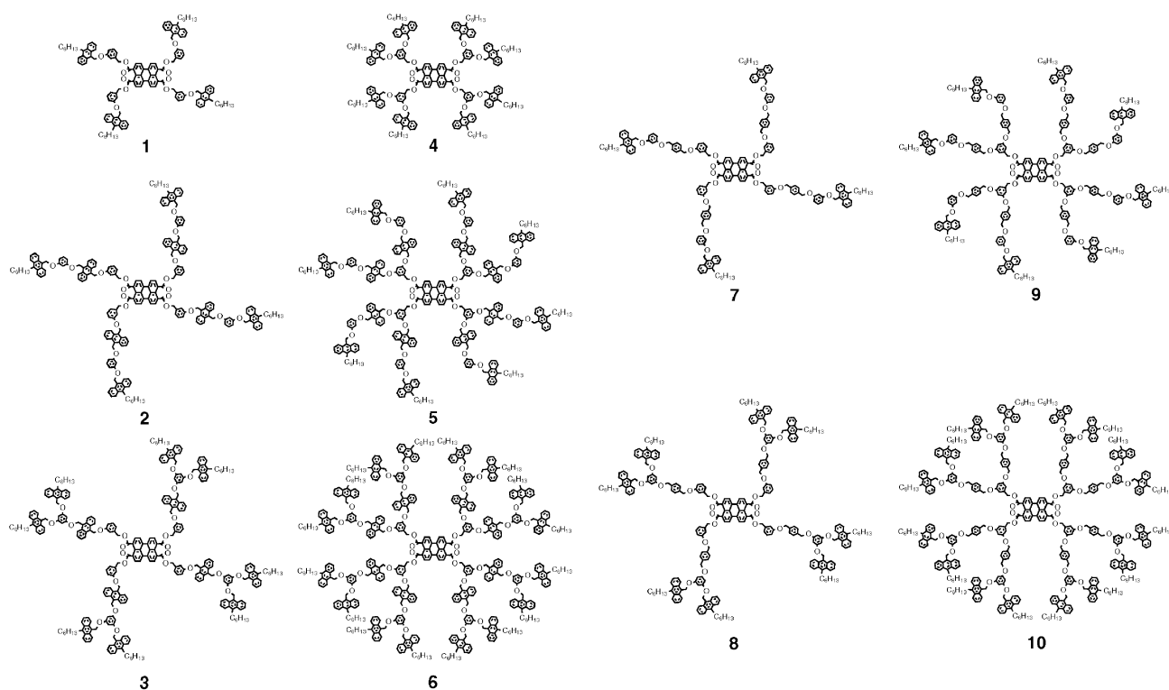
Fig. 1 Structures of 1–10.
